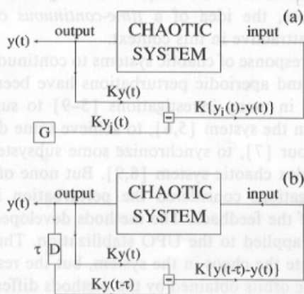
Fig. 1. Block diagram of (a) external force control, and (b) delayed feedback control. G is a special external periodic oscillator, D is a delay line.
