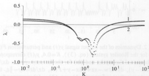
Fig. 5. Dependence of the Lyapunov exponents of the period-one and period-two UPOs of the Rossler system on the weight K of the perturbation.
