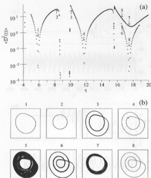
Fig. 7. (a) Dependence of the dispersion of perturbation on delay time and (b) the x - y phase portraits of the Rossler system in the post-transient regime for some values of the delay time. K=0.2 .
